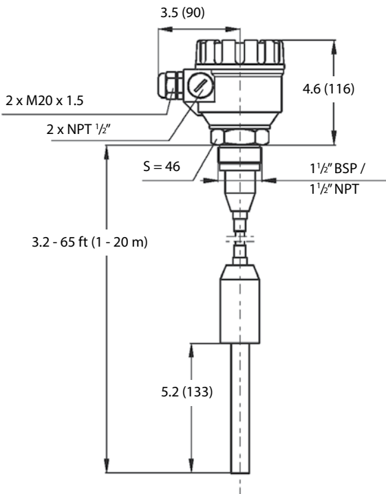
Cable Extension
