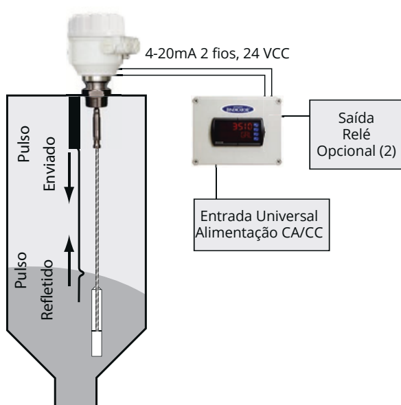
TDR-3000 com PRD1000 24 VCC
