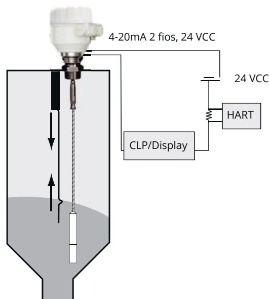
Protocolo HART TDR-3000
